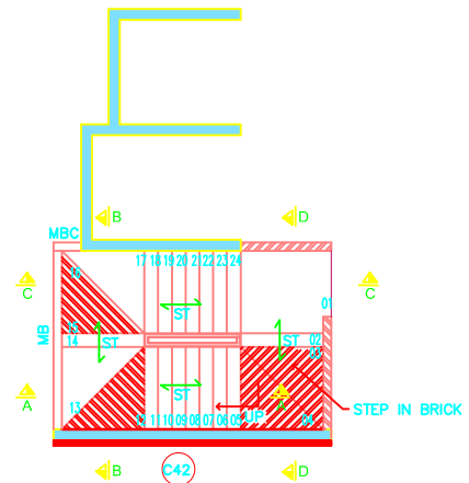
PART PLAN OF STAIRCASE
